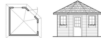
10X10 CORNER SHED DETAIL
