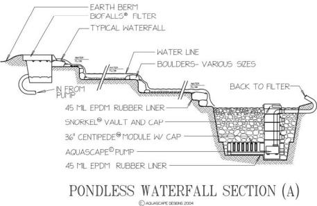
PONDLESS_A_WATERFALL
