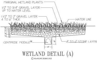
WETLAND_A_DETAIL
