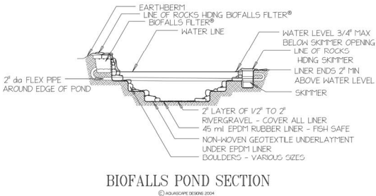
BIOFALLS_POND_SECTION
