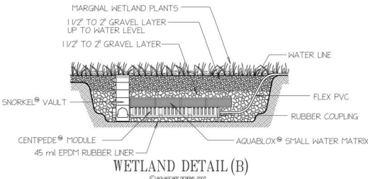
WETLAND_B_DETAIL
