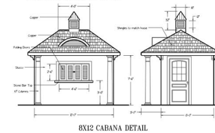
8X12 CABANA DETAIL
