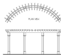
CURVED PERGOLA DETAIL
