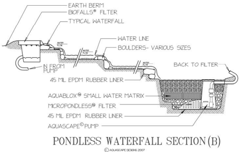
PONDLESS_B_WATERFALL
