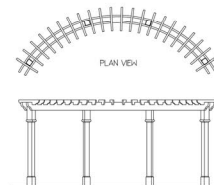
CURVED PERGOLA DETAIL
