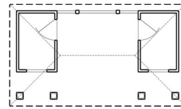
6X9 (X24) CABANA FLOOR PLAN
