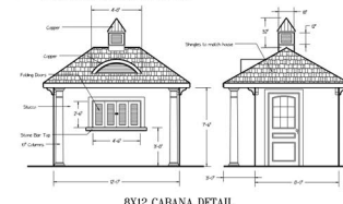
8X12 CABANA DETAIL
